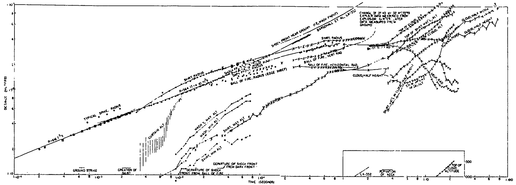
Fig. 9. Summary of optical space-time data. □ 8mm, 7110/s. W 800 F = 2 in. ⊙ 16mm, 3560/s. W 10,000 F = 6 in. ● 16mm, 655/s. N 10,000 F = 6 in. × 35mm, 107/s. N 10,000 F = 18 in. + 35mm, 24/s. N 10,000 F = 3 in. ⊗ 35mm, 119/s. W 10,000 F = 24 in.
